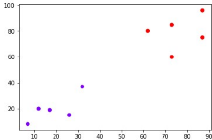
Figure 4: Dataset
