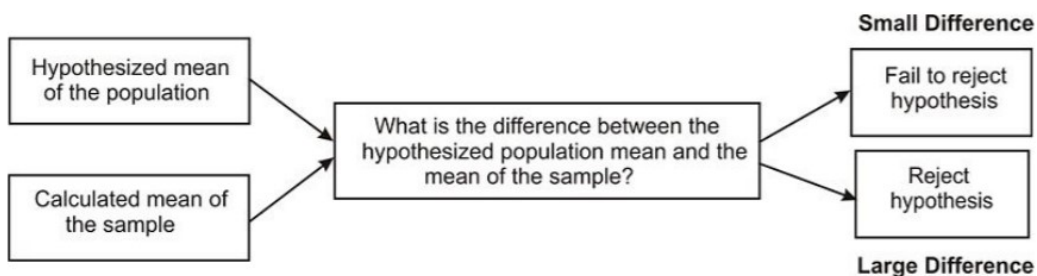
Figure 9: Hypothesis testing
