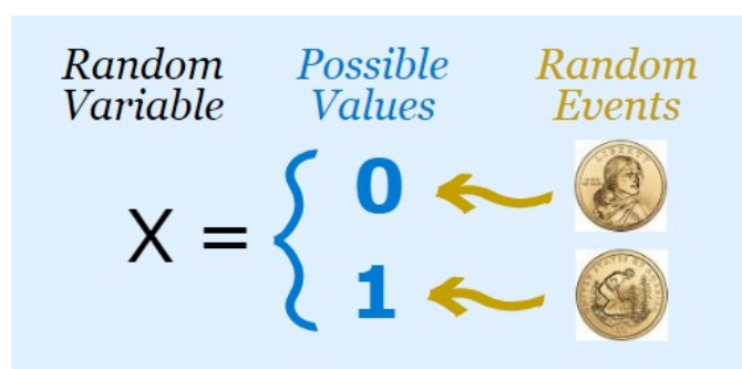
Figure 16: Random variables
