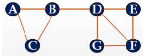
Figure 5: Distance measure graph
