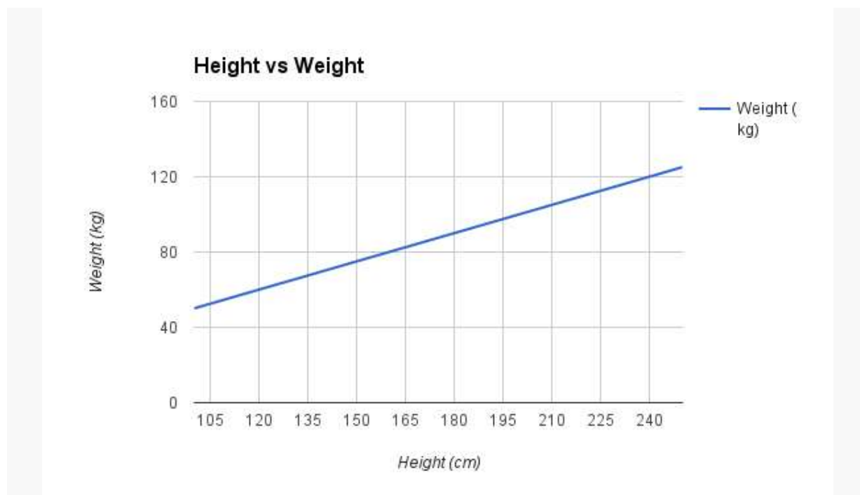
Figure 3: Sample Height vs Weight Linear Regression
