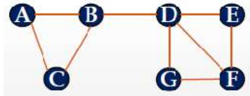
Figure 3: Hierarchical Clustering
