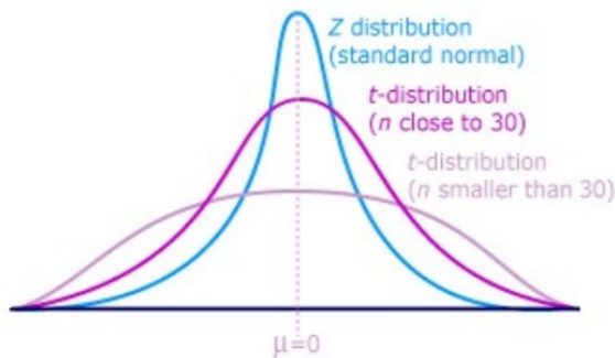
Figure 11: Distribution graph
