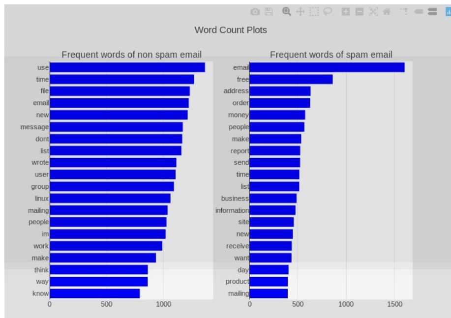
Figure 9: Bar chart visualization of 1-gram model
