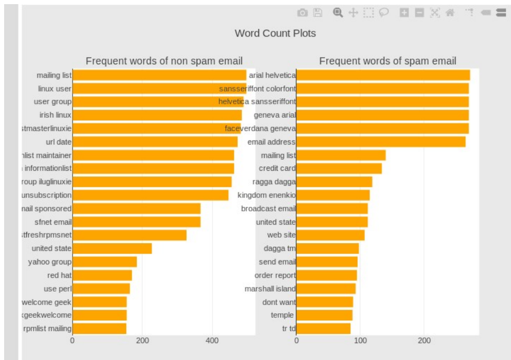
Figure 10: Bar chart visualization of 2-gram model
