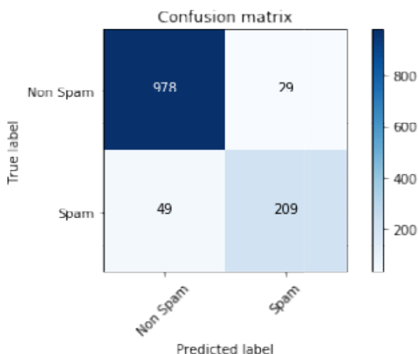
Figure 15: Confusion Matrix
