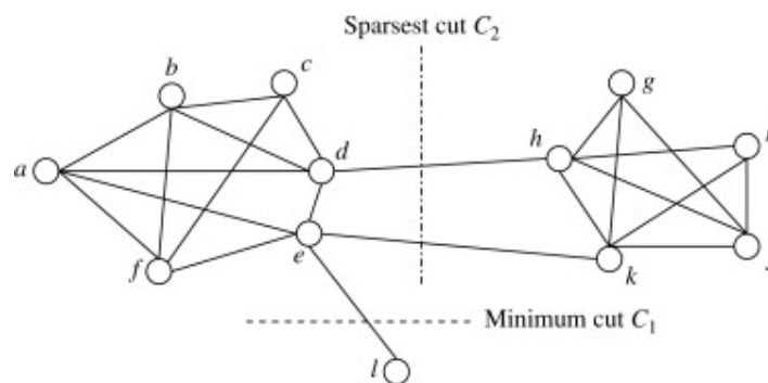
Figure 12: A graph G and two cuts
