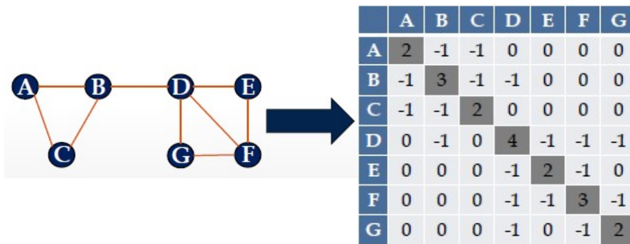
Figure 10: Laplacian Matrix
