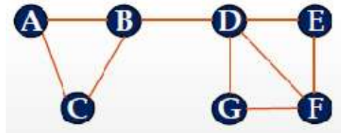
Figure 2: Distance measure for the graph
