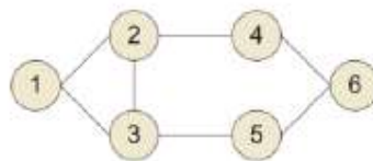
Figure 16: k-club
