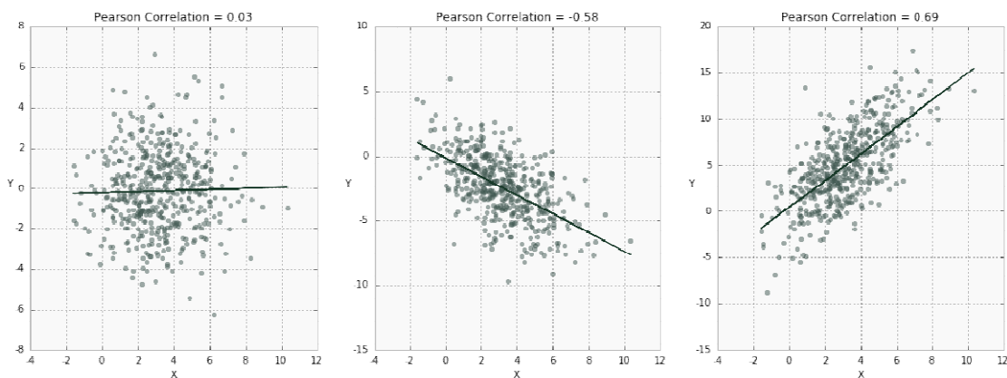
Figure 12: Pearson Correlation
