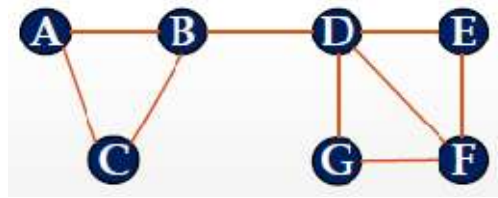
Figure 4: Example/Exercise: Calculate the betweenness
