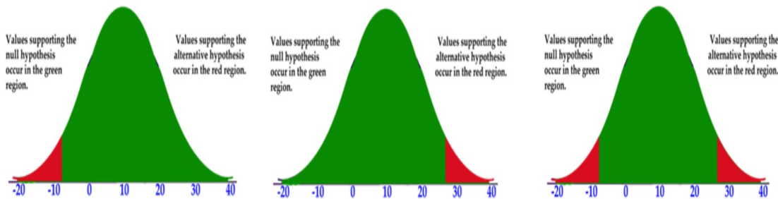
Figure 10: left, right & two-tailed tests
