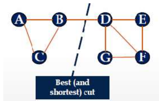
Figure 6: Partition of graph
