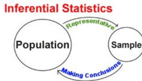
Figure 7: Inferential statistics
