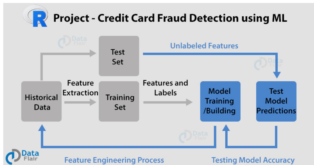
Figure 21: Layout of Credit Card Fraud Detection Project in R
