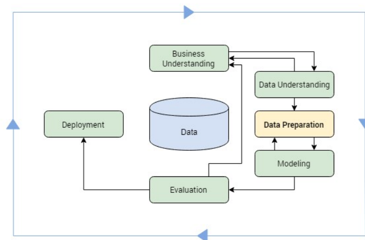
Figure 16: Data Munging
