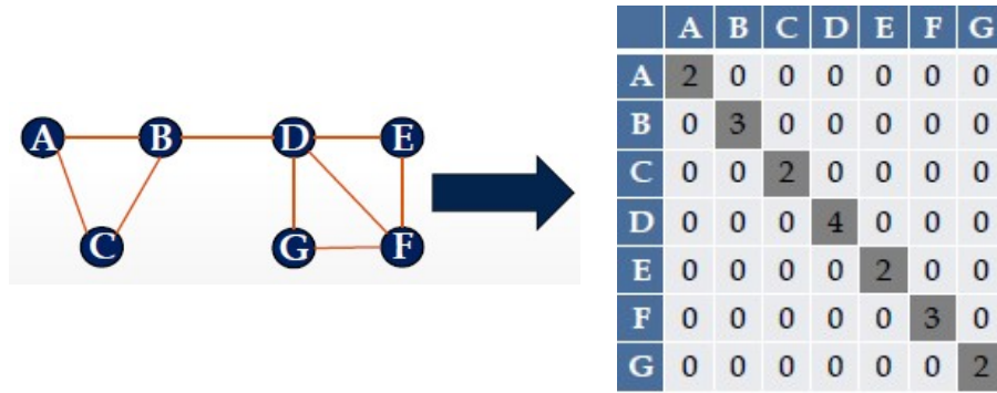
Figure 9: Degree Matrix
