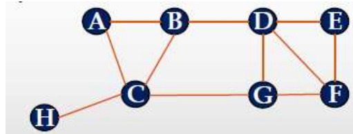
Figure 7: Normalized cuts graph
