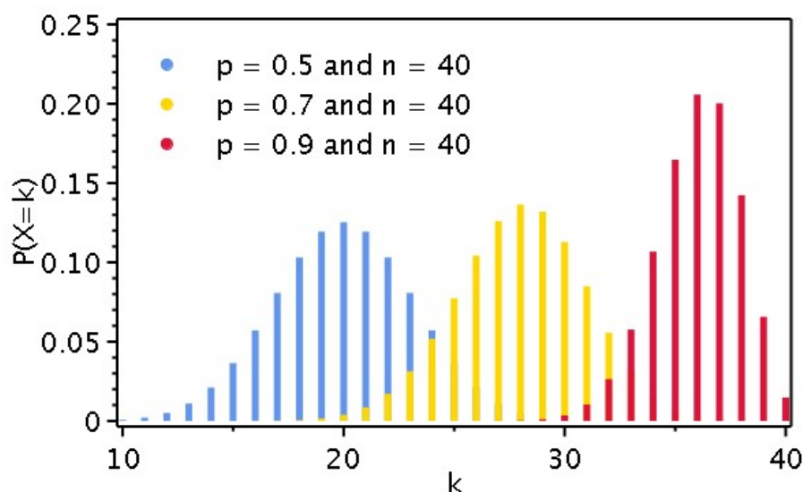
Figure 17: Probability Distributions
