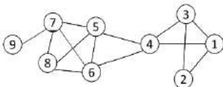
Figure 15: k-clique
