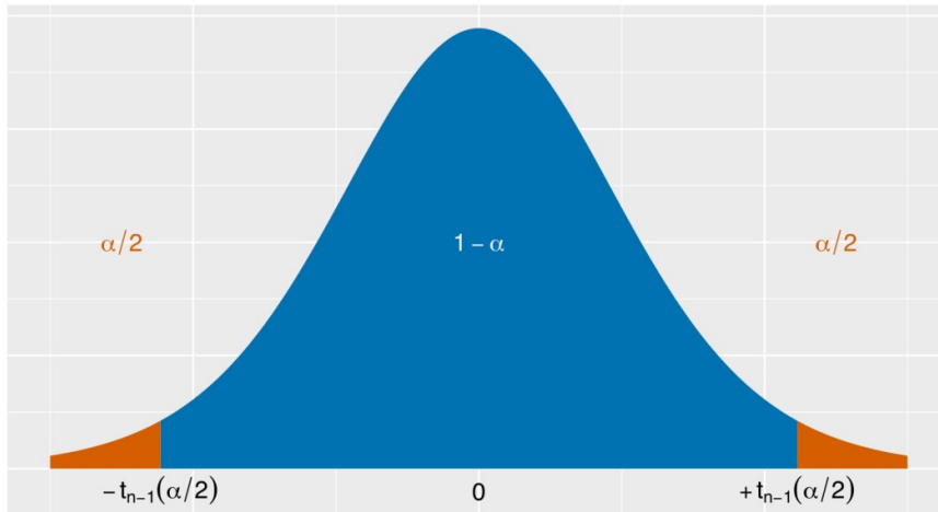
Figure 8: Confidence intervals graph
