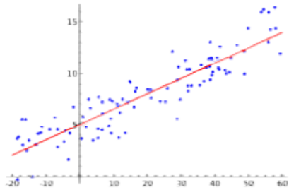
Figure 13: Regression
