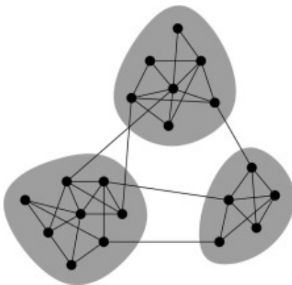
Figure 11: Structure of a cluster
