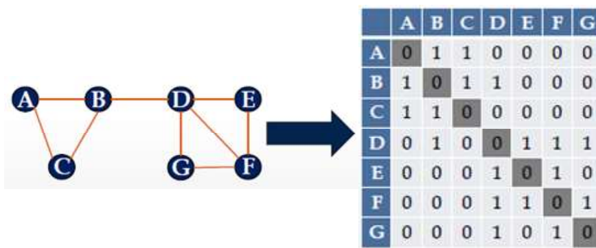
Figure 8: Adjacency Matrix
