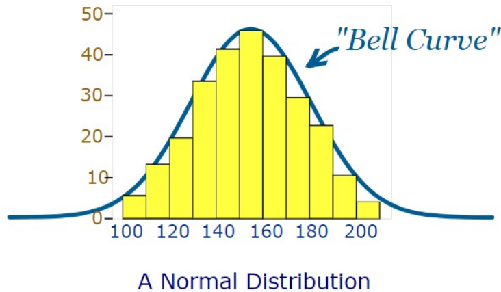
Figure 18: Normal Distribution
