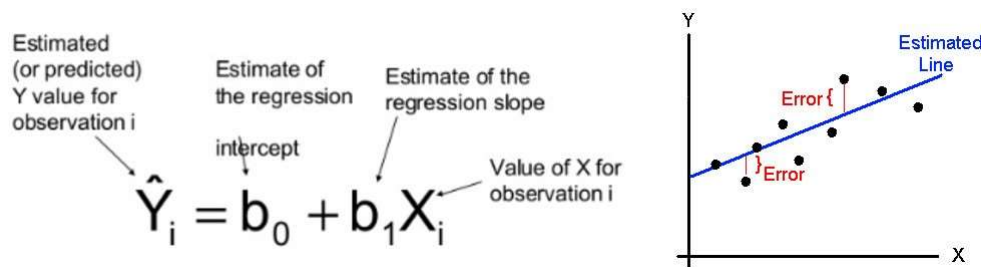
Figure 13: Simple Regression
