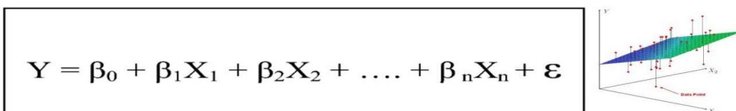
Figure 14: Multiple Regression
